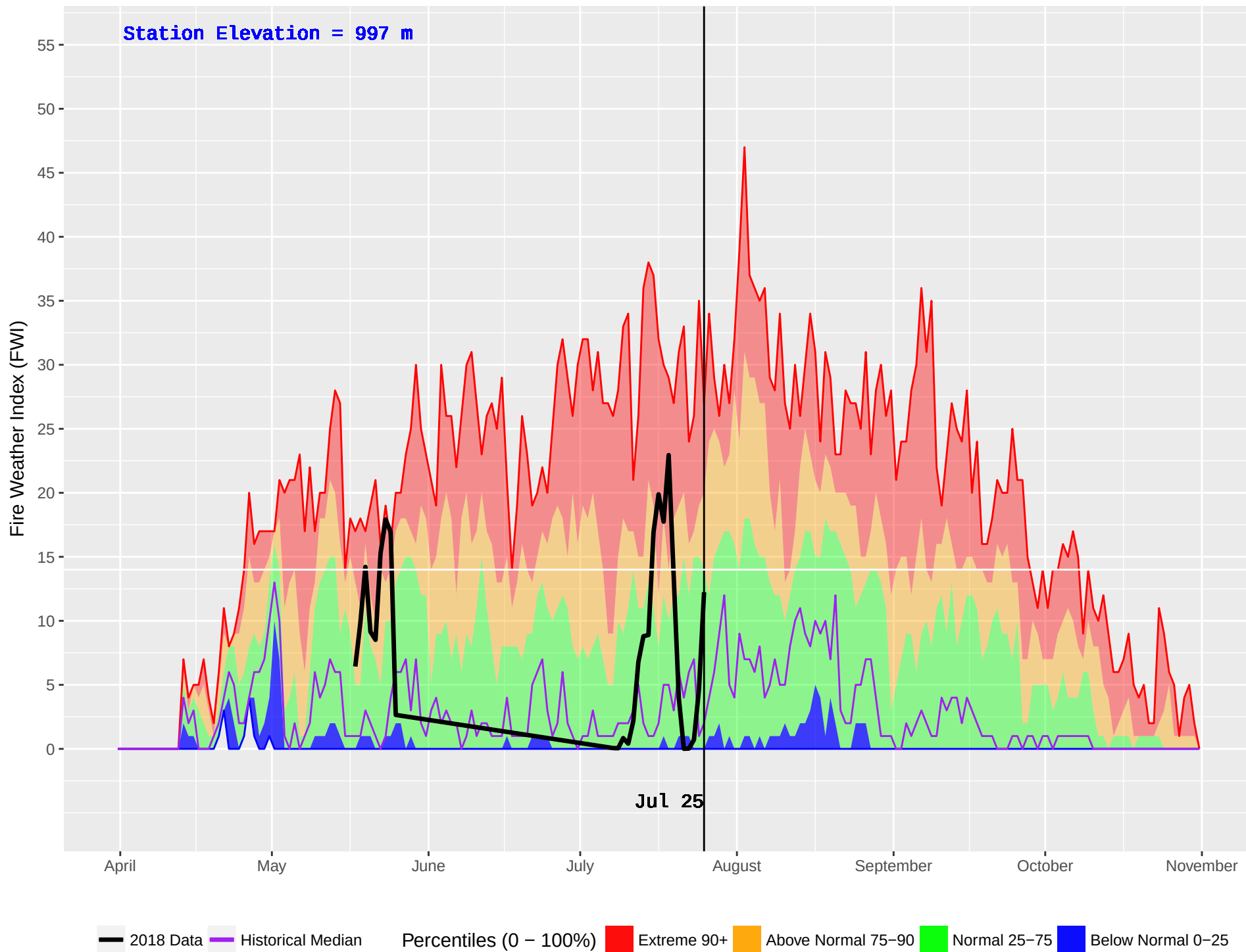
JERRY (190) : Historical (1988–2016) and Current (2018) Noon Fire Weather Index (FWI)
