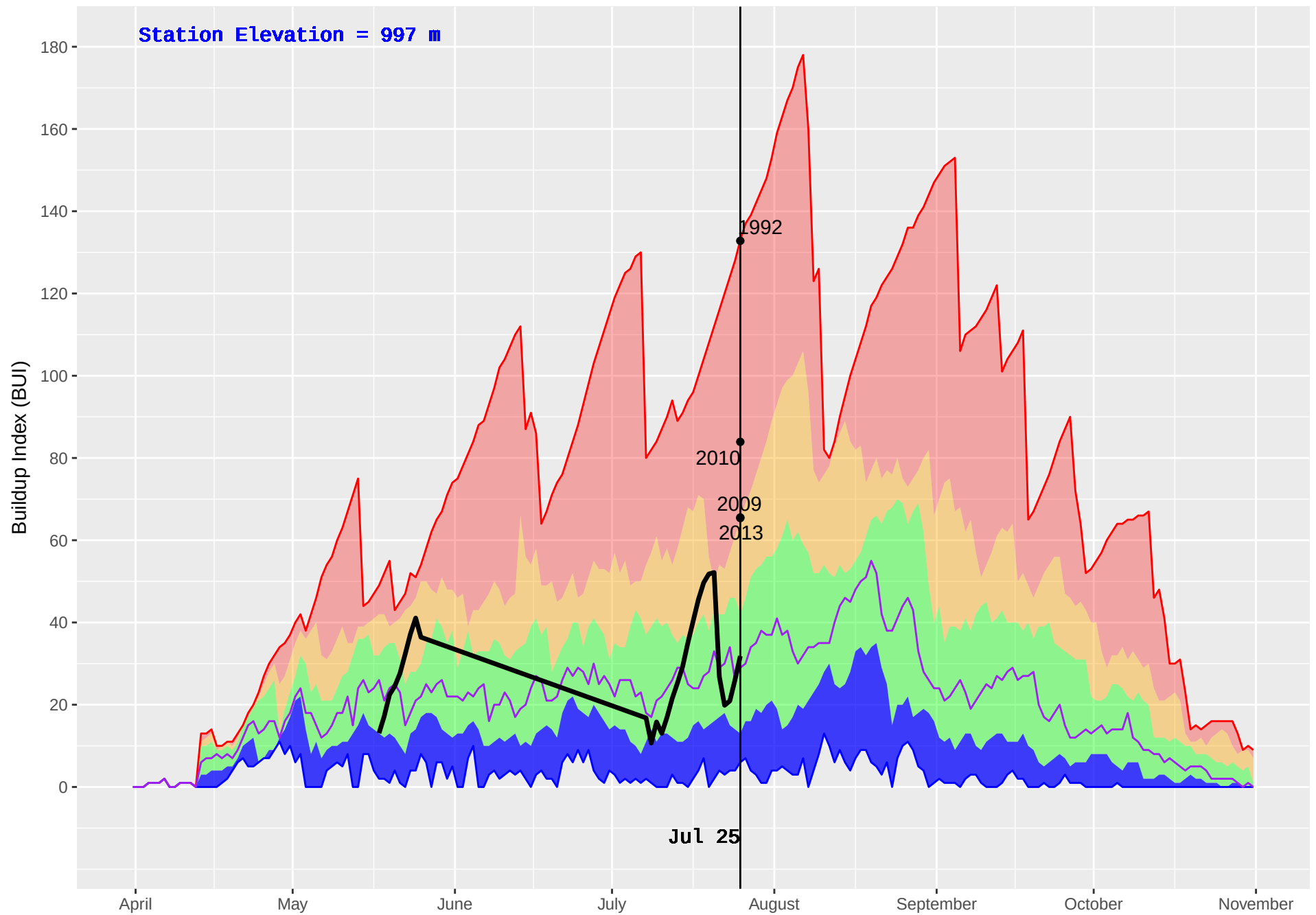
JERRY (190) : Historical (1988–2016) and Current (2018) Noon Buildup Index (BUI)
