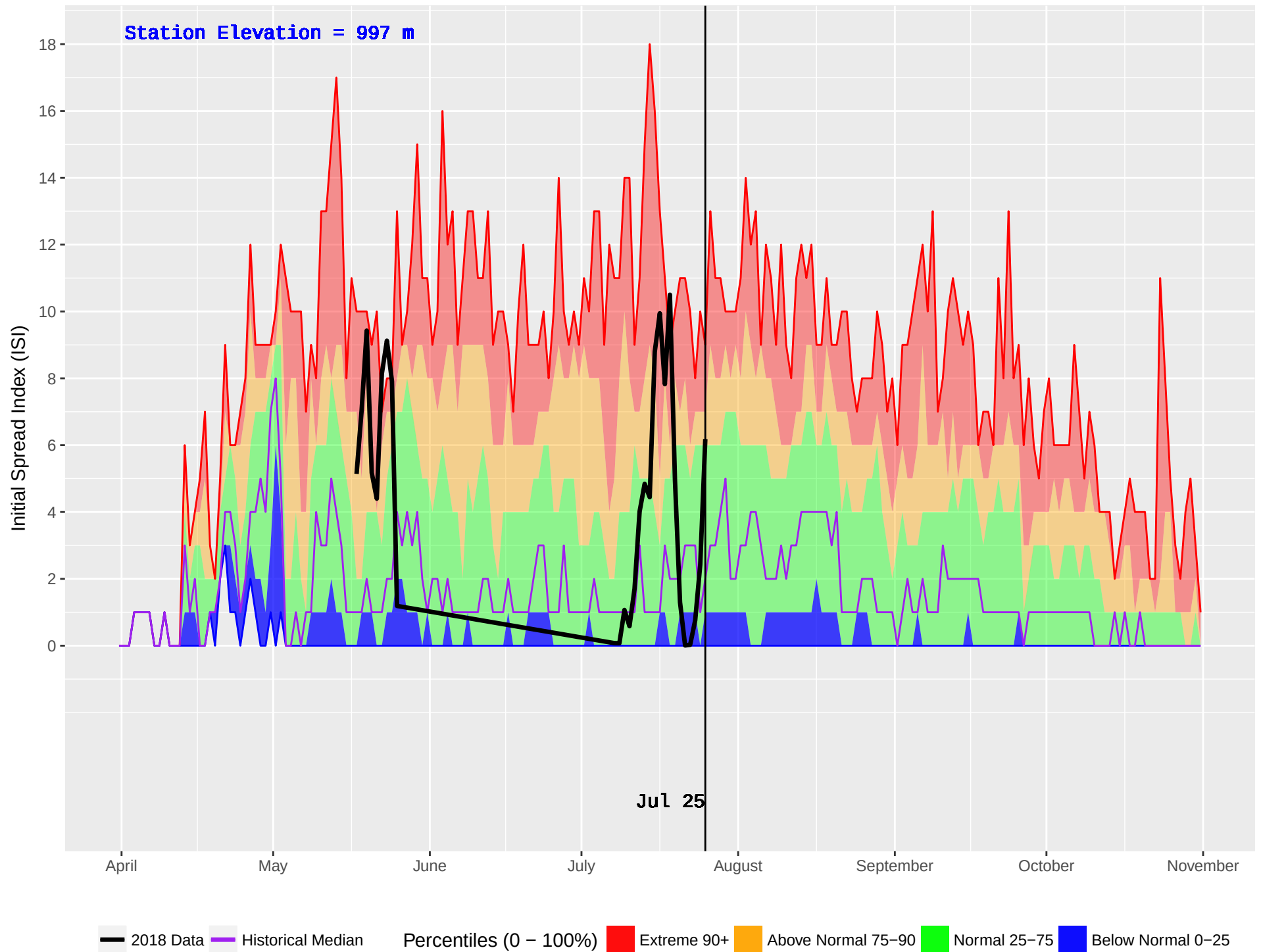
JERRY (190) : Historical (1988–2016) and Current (2018) Noon Initial Spread Index (ISI)
