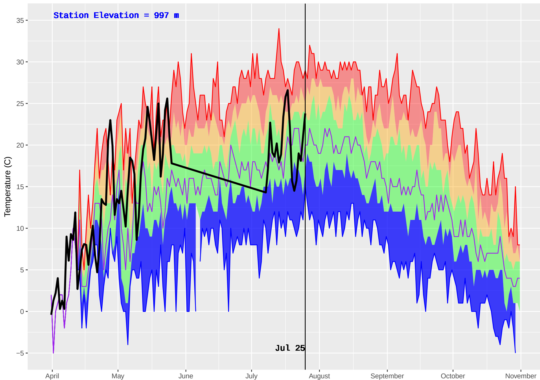
JERRY (190) : Historical (1988–2016) and Current (2018) Noon Temperature
