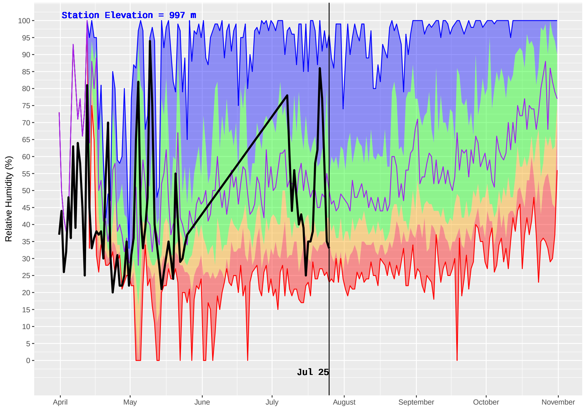
JERRY (190) : Historical (1988–2016) and Current (2018) Noon Relative Humidity
