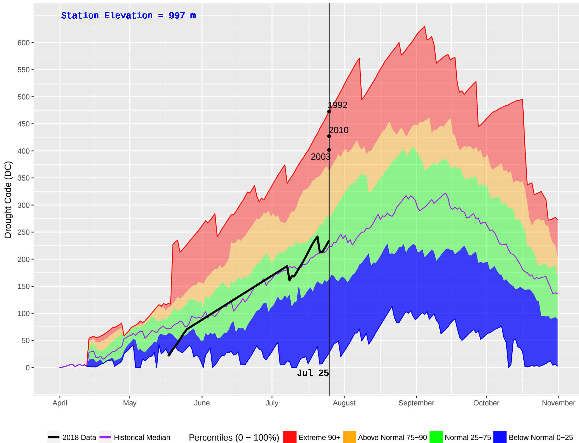
JERRY (190) : Historical (1988–2016) and Current (2018) Noon Drought Code (DC)
